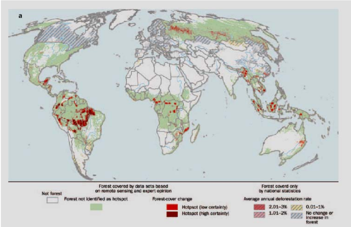
Fig. 1: Main area of forest-cover changes between 1980 and 2000. From Lepers et al. (2005).
