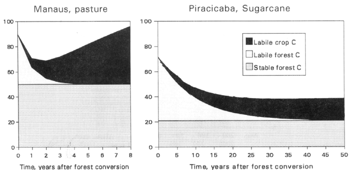
Fig. 6: Soil organic matter dynamics in Oxisols after forest conversion to pastures and sugar cane. Graphs based on fitted regression models. From van Noordwijk et al. (1997) based on PhD work by C.C. Cerri in Brazil.
