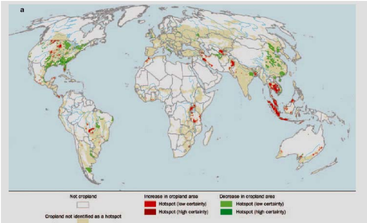
Fig. 2: Main area change in cropland extent between 1980 and 1990. From Lepers et al. (2005).
