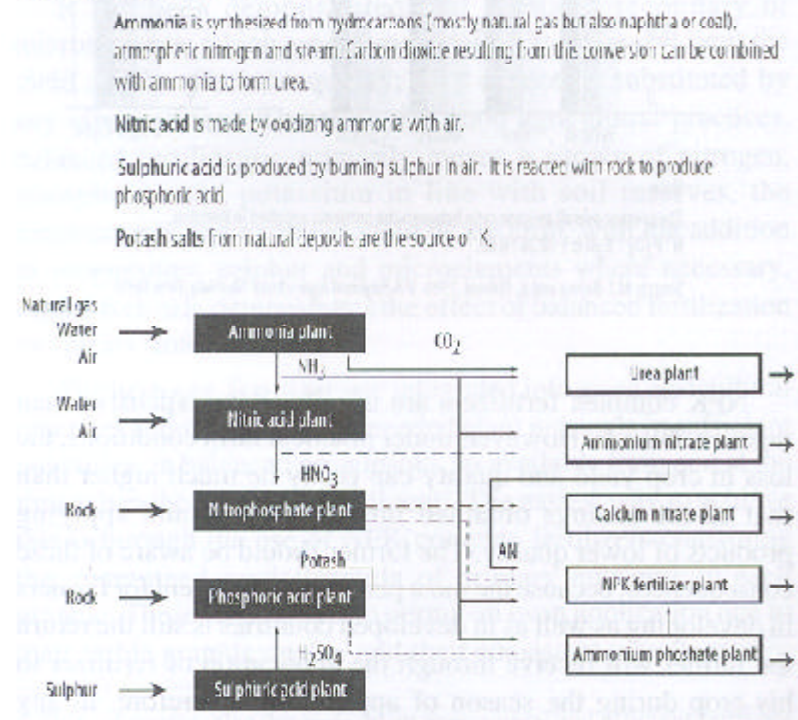
Figure 7. Diagram of fertilizer production routes
